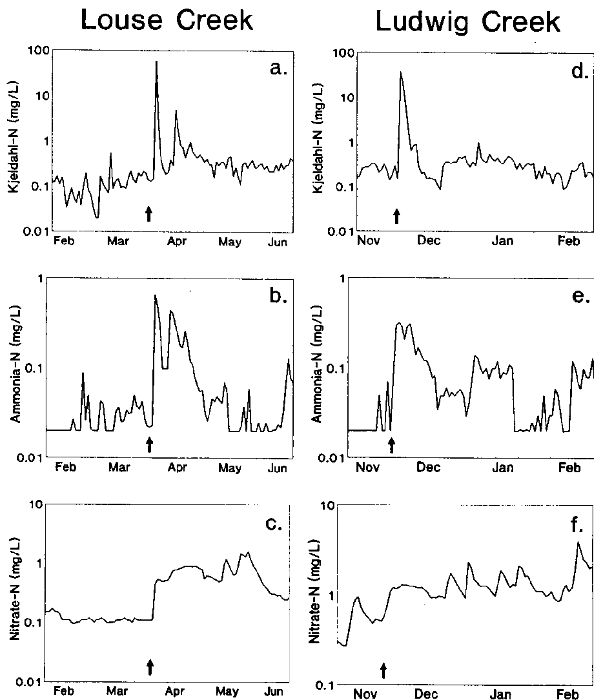
Figure 2. Changes in dissolved nitrogen species after urea application (224 kg N/ha) in Louse Creek, a midelevation stream in the Cascade Range, and Ludwig Creek, a low elevation stream in the Coast Range. Arrows indicate time of fertilization. From P. Bisson and B. Fransen, unpublished.
